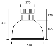
LED High-Bay B 150W
